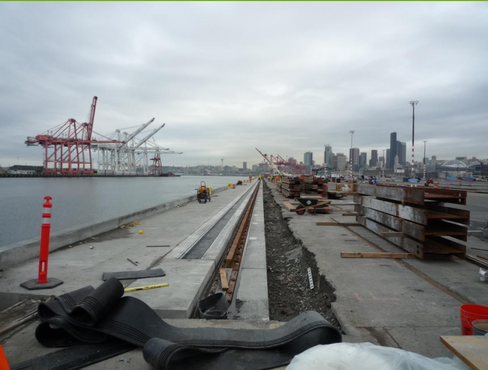
Waterside Crane Beam work March 2009
