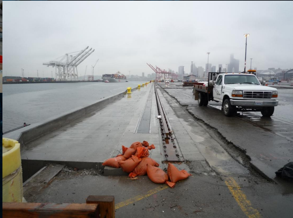
Waterside Crane Beam work April 2009
